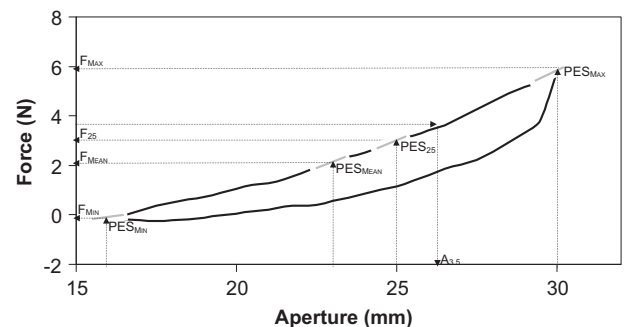
Fig. 2. The means of cycles 3, 4 and 5 are presented. The PES parameters are given by the slope of the curve at the selected points. Passive parameters extracted from the force-aperture curve are illustrated: force ( F_{\text{MIN}} ) and passive elastic stiffness ( \text{PES}_{\text{MIN}} ) at minimal aperture, force ( F_{\text{MAX}} ) and passive elastic stiffness ( \text{PES}_{\text{MAX}} ) at maximal aperture, force ( F_{\text{MEAN}} ) and passive elastic stiffness ( \text{PES}_{\text{MEAN}} ) at mean aperture, force ( F_{25} ) and passive elastic stiffness ( \text{PES}_{25} ) at the common aperture of 25 mm, aperture at a common force of 3.5 N ( A_{3.5} ) and hysteresis (area between the lengthening and shortening curves).
