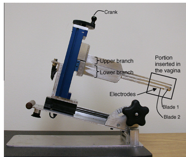
Fig. 1. The lower branch comprises two blades. The passive properties were recorded with blade 2, which is located at the level of the PFMs. In the picture, the speculum is opened to the minimal aperture, which corresponds to a vaginal antero-posterior diameter of 15 mm (distance between lower and upper branches). As also shown, the speculum can be tilted to respect woman's natural vaginal orientation; the portion of the speculum inserted into the vagina corresponds to 6 cm.
